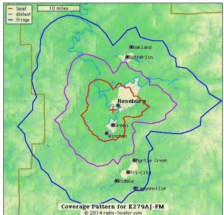
Roseburg Translator 103.7
