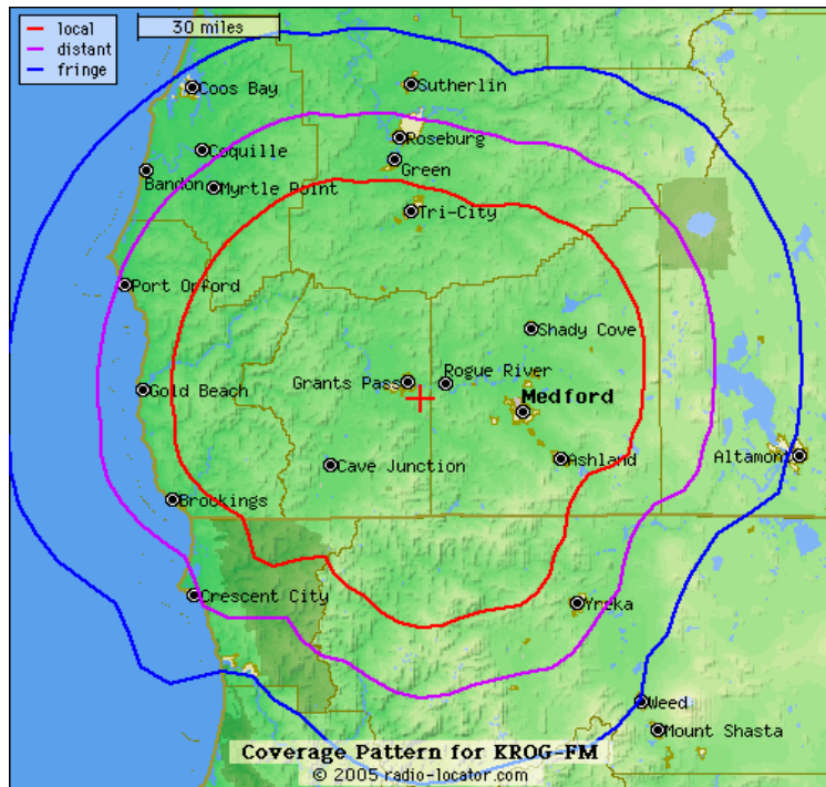
Main Transmitter 96.9
