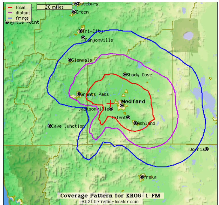
Additional Booster 96.9
